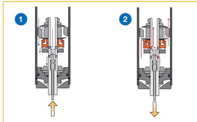
FIGURE 1: (Compression flow) At low shaft speeds, oil flows mostly through the shaft jet bleed (lower dotted arrow). At high shaft speeds, oil flows mostly through the compression ports in the piston (upper dotted arrow). At intermediate shaft speeds, which are very critical for comfort, or during sudden shaft accelerations, oil can also escape through the compression ports in the DFV (solid arrow), increasing comfort.
